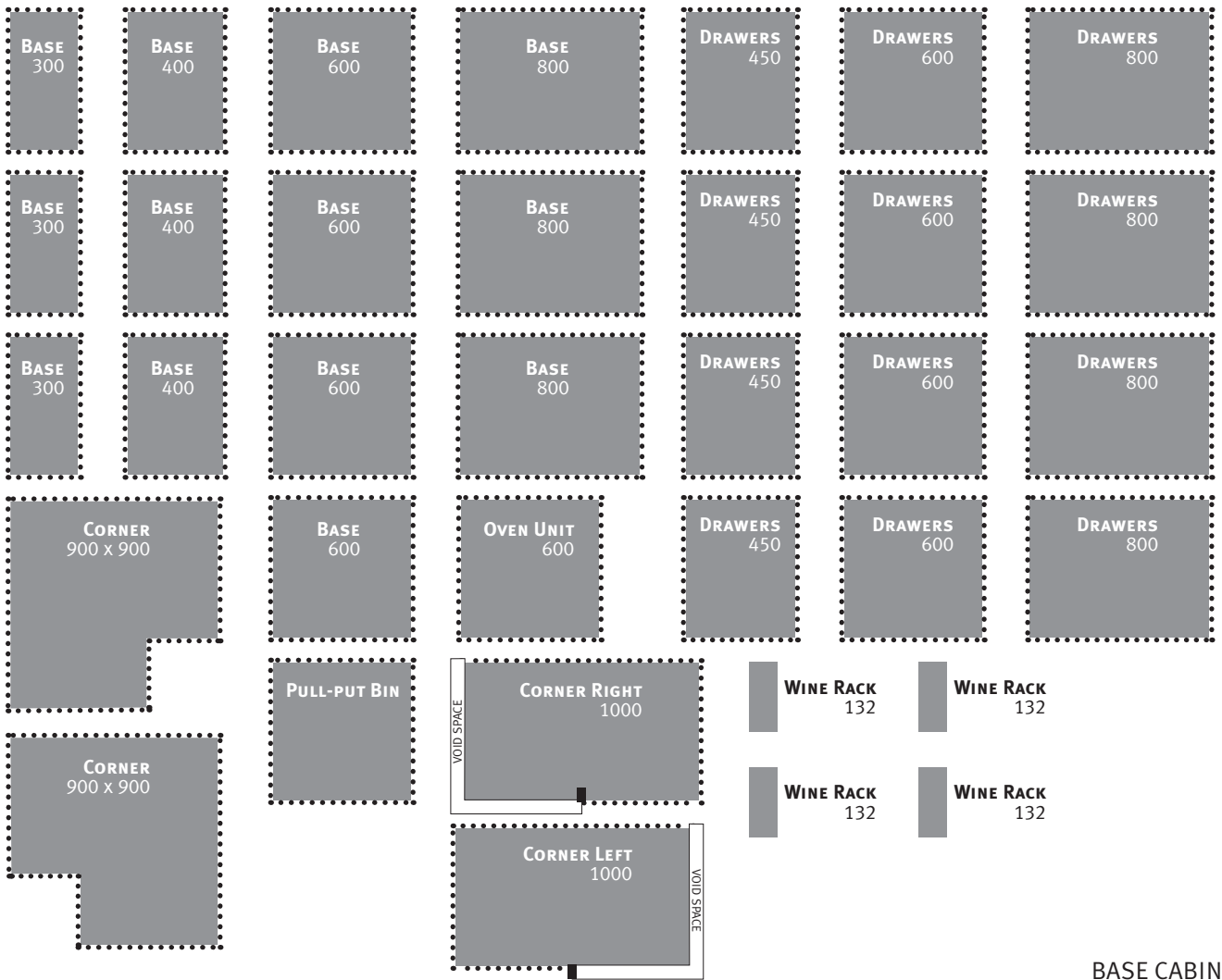
BASE CABINETS
